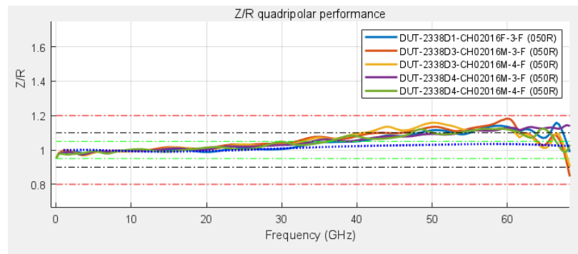
Fig. 18 - - Frequency response of a 50 Ω; CHA02016 after AEC-Q200 high temperature exposure vs. datasheet values
