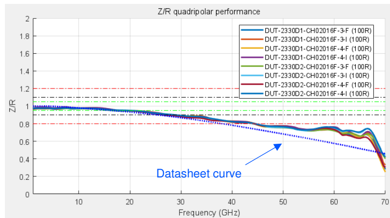
Fig. 15 - Frequency response of a 100 \Omega ; CHA02016 before (-I) and after (-F) a AEC-Q200 biased humidity test
