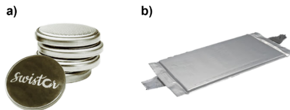
Fig. 5. a) Coin cell format with capacitance from 0.2 to 2 F. b) Pouch cell with capacitances up to 5 F.
