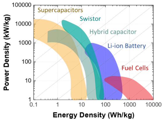
Fig. 2. Ragone plot showing the trade-offs between energy density and power density for the different electrochemical energy storage devices including Swistor capacitors.
