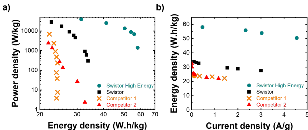
Fig. 9. Comparison plots normalized by electrode material. a) Ragone plot comparing energy and power density and b) energy density over current density for the two types of Swistor capacitors and two commercially available EDLC.
