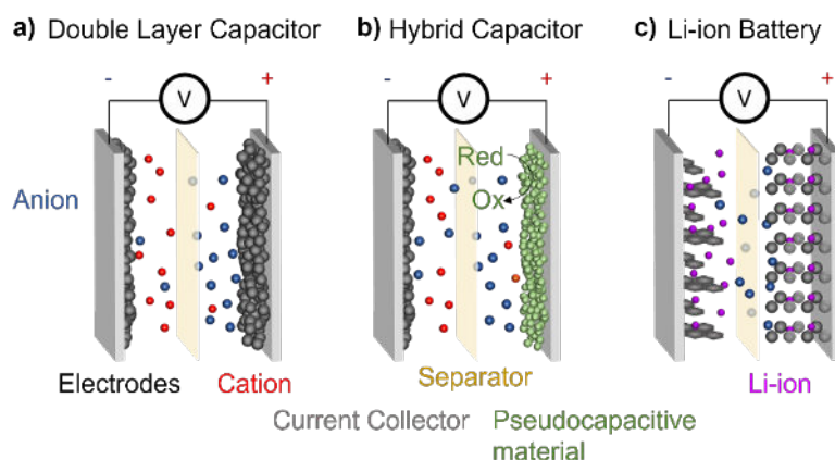
Fig. 1. Representation of electrochemical devices for energy storage. a) Symmetrical electrochemical double layer capacitor. b) Redox enhanced hybrid electrochemical double layer capacitor. c) Lithium-ion battery.
