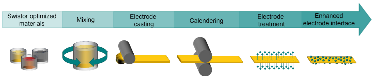
Fig. 3. Process flow for electrode manufacturing. Starting from raw materials, the electrode components are mixed, and the electrode is cast into a foil that is later densified by calendering. After this step the electrodes are subjected to a specific treatment to improve the interface with the electrolyte.
