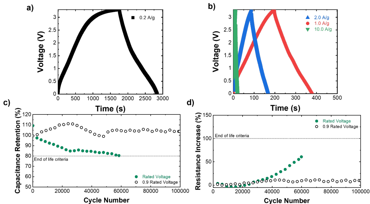
Fig. 7. Performance metric of a 0.2 F of a Swistor coin cell at different current ranges densities normalized by electrode mass. a) Charge-discharge curves for low current densities, b) charge-discharge curves for high currents densities. Lifetime performance at rated voltage of 3.3 V and 3 V (0.9 x rated voltage) following continuous cycling showing c) capacitance retention and d) resistance increase.
