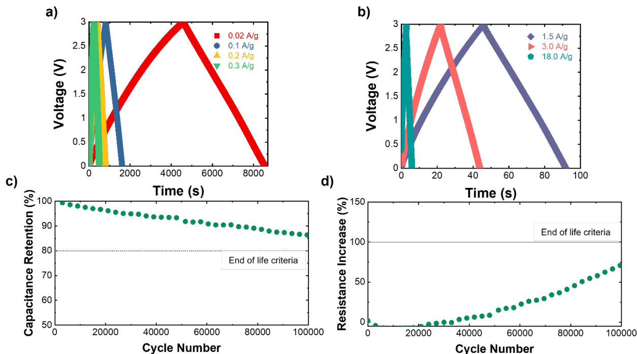
Fig. 6. Performance for small coin cell EDLC supercapacitors of 0.15 F at 3V at different current ranges densities normalized by electrode mass. a) Charge-discharge curves for low current densities, b) Charge-discharge curves for high currents densities. Durability upon continuous cycling at 3 V indicating c) capacitance retention and d) resistance increased.
