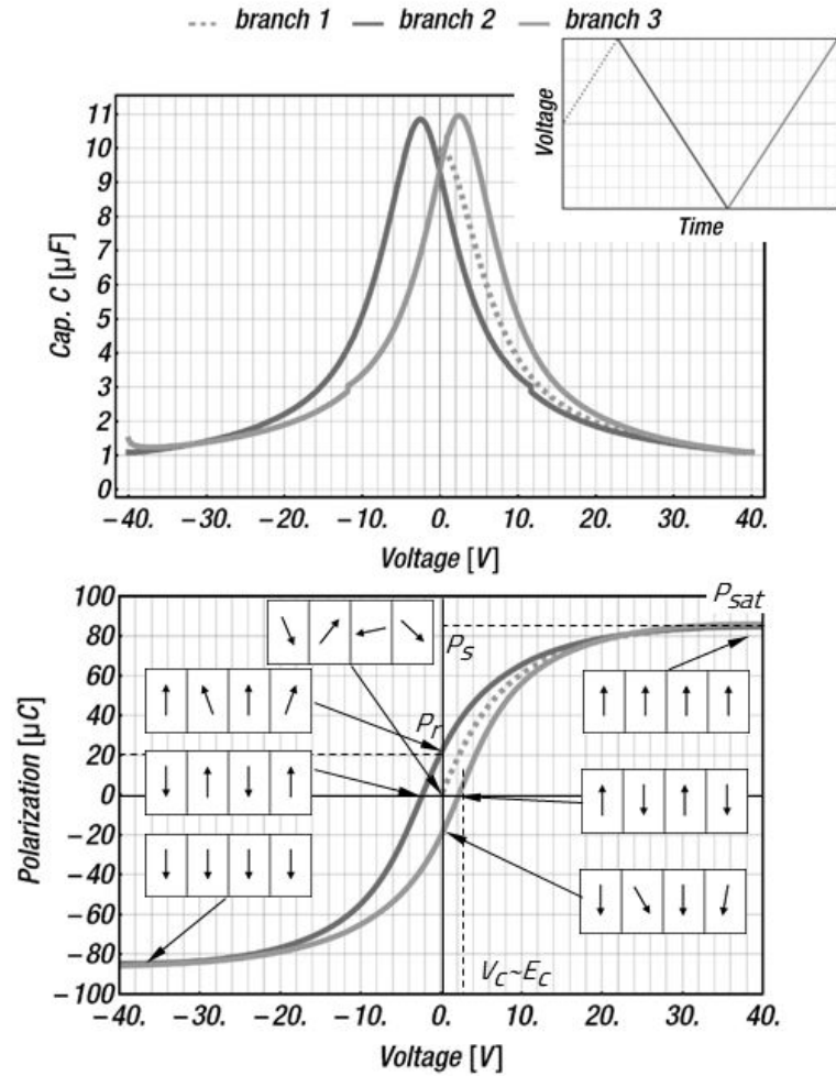
Figure 2 TOP: Measured capacitance-voltage characteristics of 10 \mu\text{F} MLCC, for a dc voltage cycle, shown in the inset graph. BOTTOM: Polarization-voltage characteristics with corresponding schematic depiction of dipole orientation.
