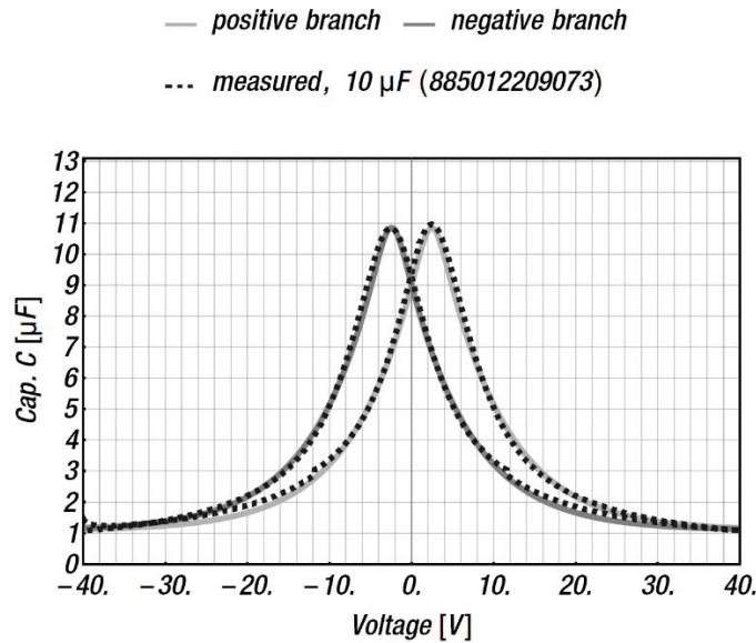
Figure 3 Measured capacitance-voltage characteristic of 10 \mu\text{F} MLCC with the corresponding fit of equation 1. Dimensionless numerical fit-parameters: a=10.85 , b=1.3 , c=0.17 , C_S=1.09 , V_C=2.5 .
